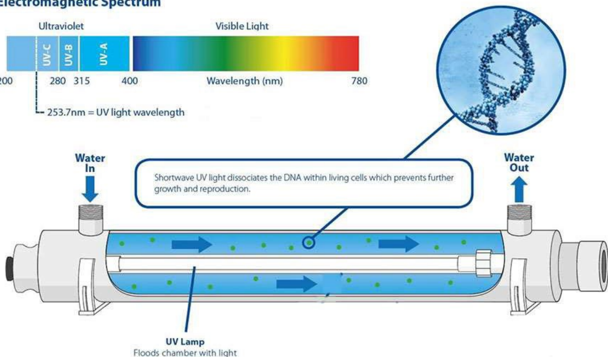
Electromagnetic Spectrum
