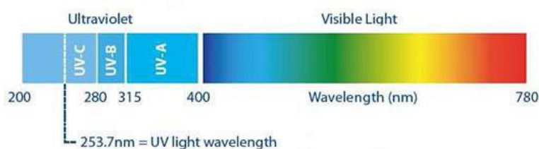
Electromagnetic Spectrum
